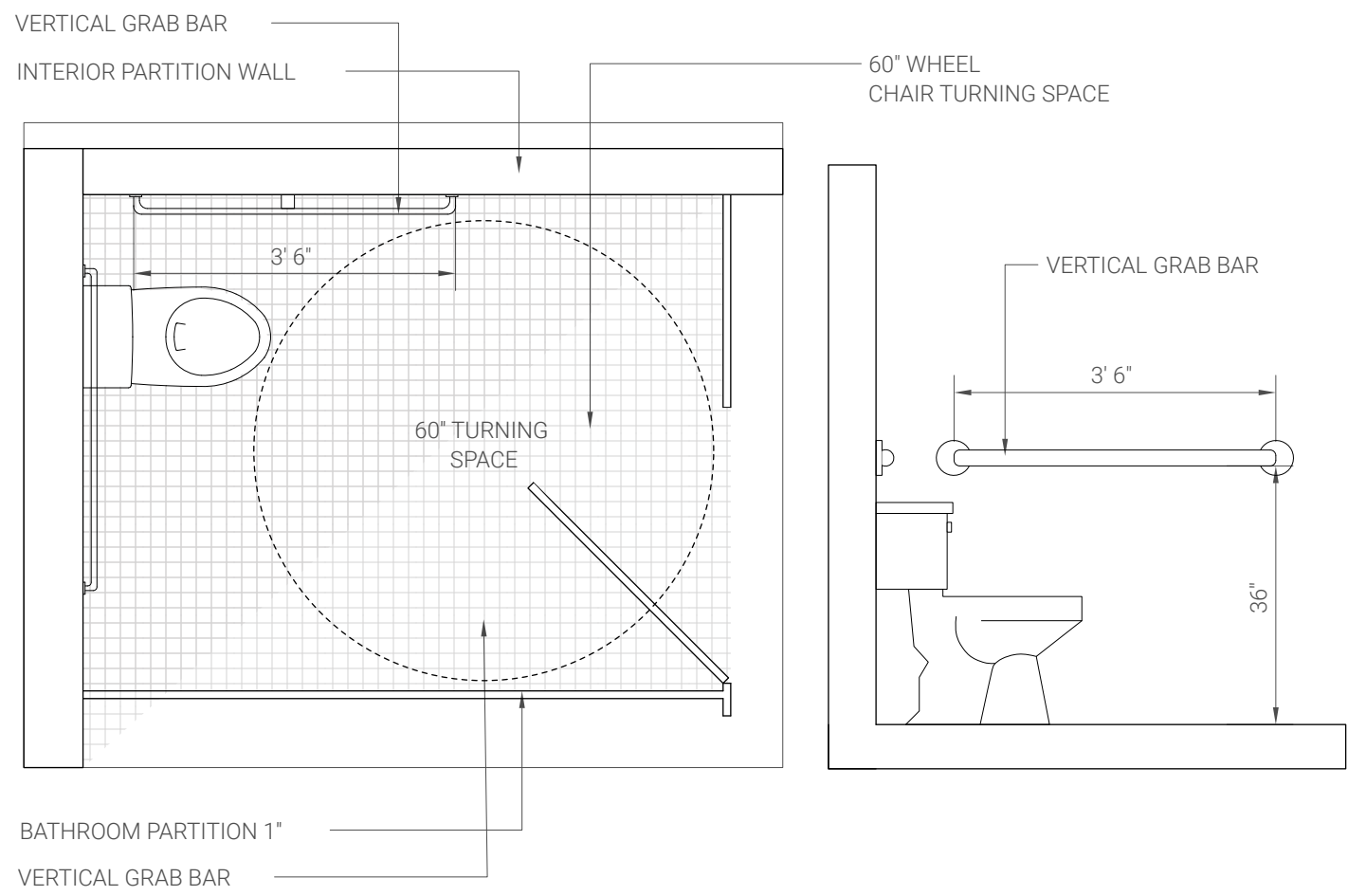
ADA BATHROOM DETAIL SCALE: 1/2" = 1'-0"
