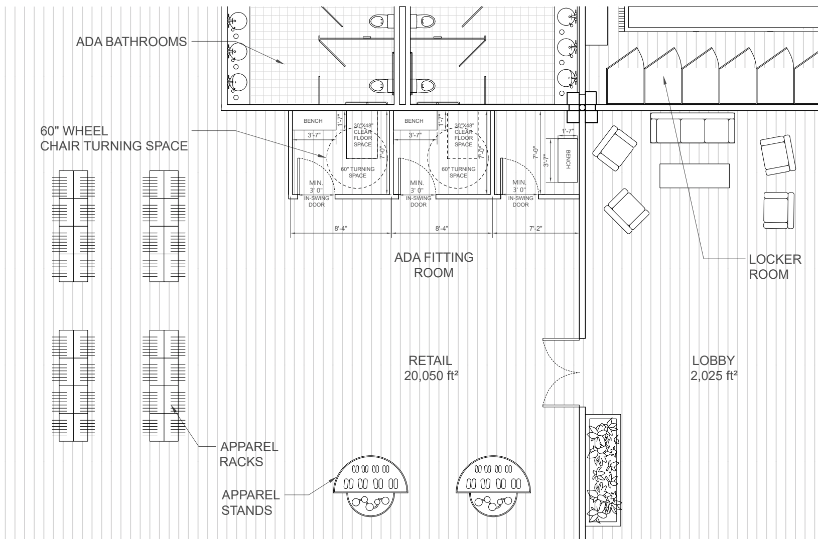
ADA FITTING ROOMS SCALE: 1/8" = 1'-0"
